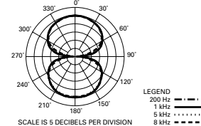
polar pattern
