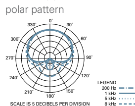
polar pattern
