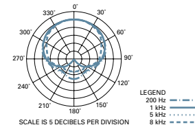
polar pattern
